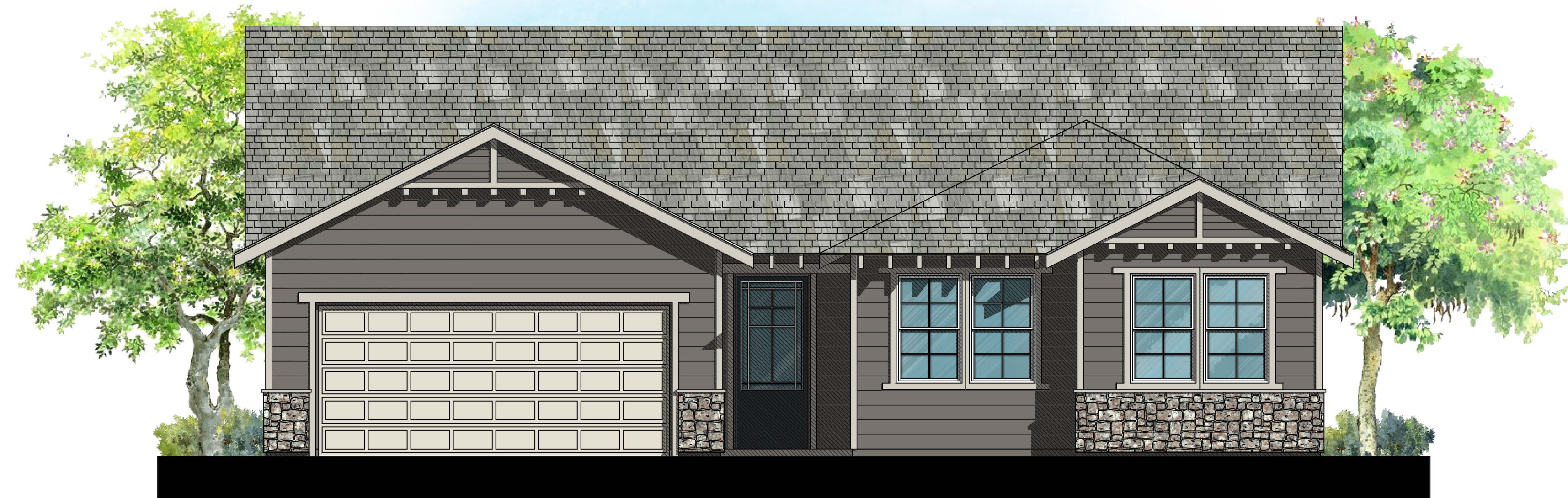
2 FRONT ELEVATION
