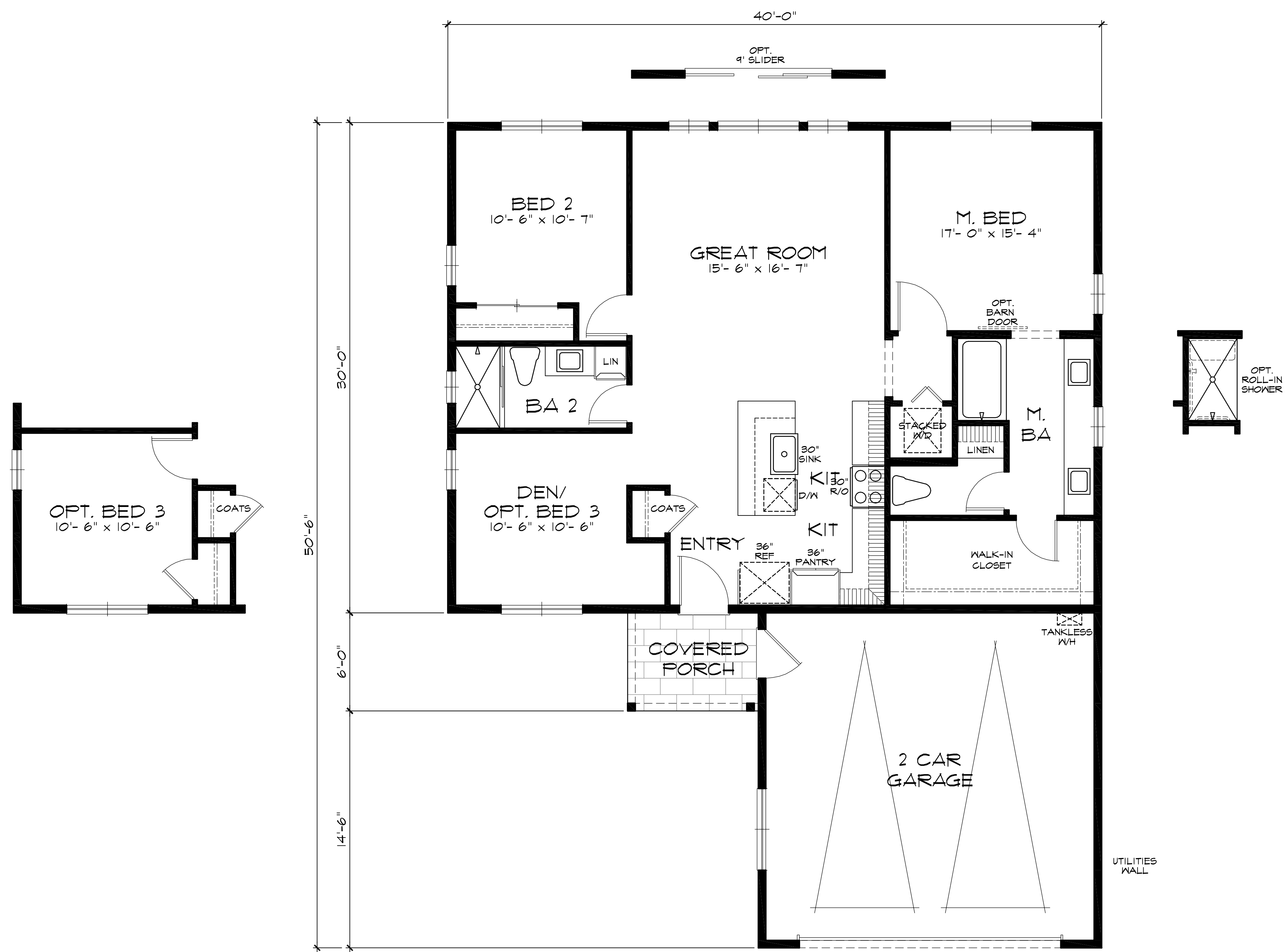
FLOOR PLAN FARMHOUSE SCALE: 1/4" = 1'-0"
